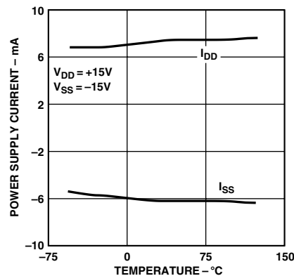
Figure 27. Power Supply Current vs. Temperature
