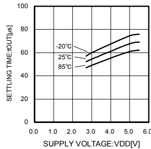
Fig.16 Settling time
