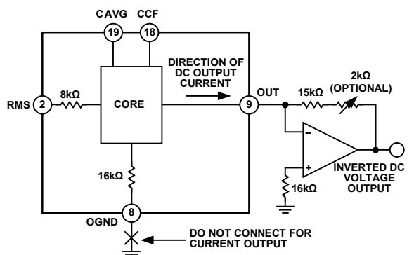
Figure 37. Connections for Current Output Showing Voltage Inversion
