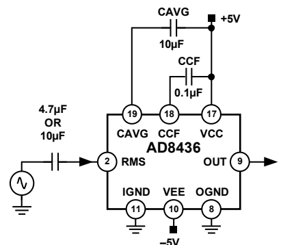
Figure 31. Connection for Additional Crest Factor Performance
