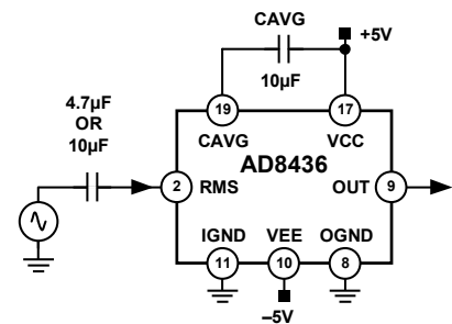
Figure 30. Basic Applications Circuit
