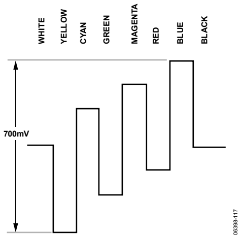
Figure 116. Pb Levels—NTSC
