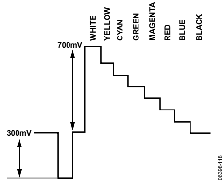
Figure 117. Y Levels—PAL
