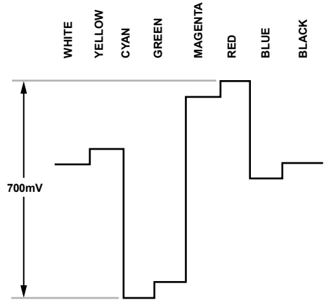
Figure 118. Pr Levels—PAL
