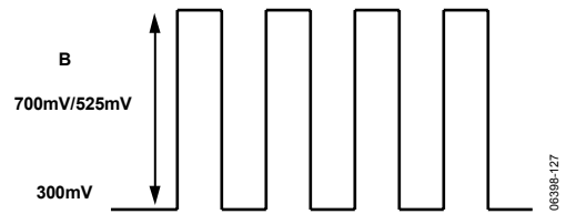
Figure 126. HD RGB Output Levels—RGB Sync Disabled
