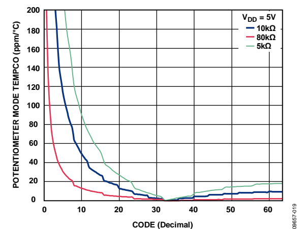
Figure 19. Potentiometer Mode Tempco \Delta R_{WB}/\Delta T vs. Code
