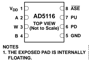
Figure 7. Pin Configuration
