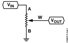
Figure 43. Potentiometer Mode Configuration
