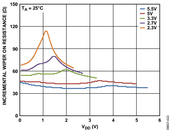
Figure 22. Incremental Wiper on Resistance vs. V_{DD}
