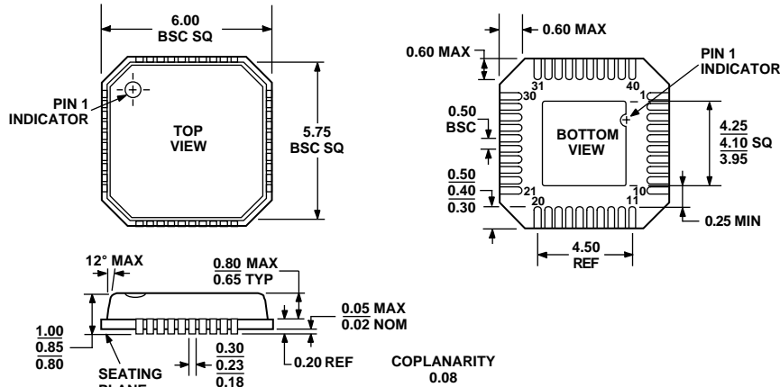
Figure 81. 40-Lead Lead Frame Chip Scale Package [LFCSP] (CP-40) Dimensions shown in millimeters
