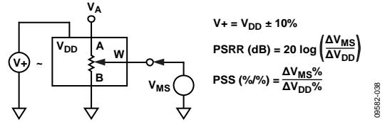
Figure 38. Power Supply Sensitivity (PSS, PSRR)
