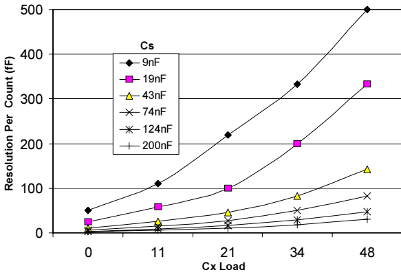
Figure 7-4 Typical resolution vs Cx & Cs; Vdd = 3.0 Volts
