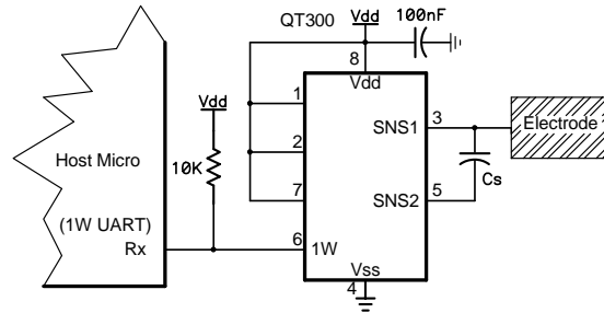
Figure 1-2 Basic QT300 Circuit in UART mode.
