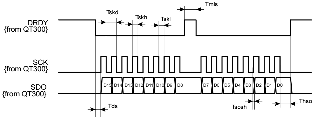
Figure 7-2 SPI Master Mode
