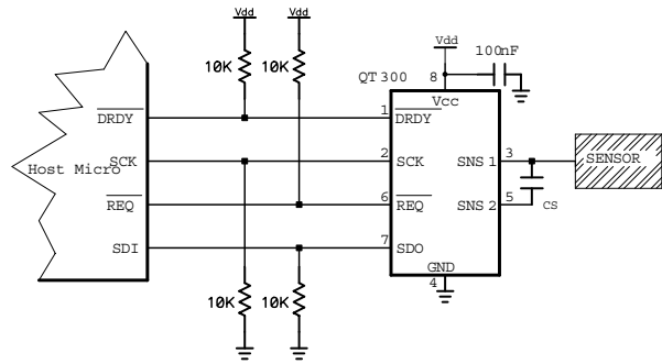
Figure 1-1 Basic QT300 Circuit in SPI mode.
