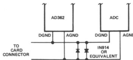
Figure 6. Ground-Fault Protection Diodes
