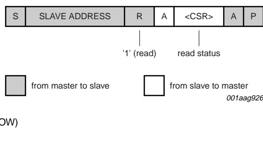
Fig 5. Host reads TDA9950 Status Register - without setting address pointer (was at 0)
