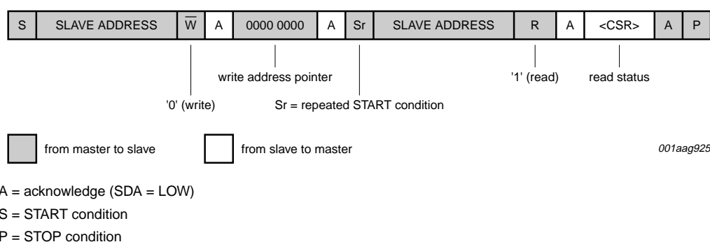
Fig 4. Host reads TDA9950 Status Register - after setting address pointer
