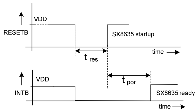
Figure 22 Hardware Reset
