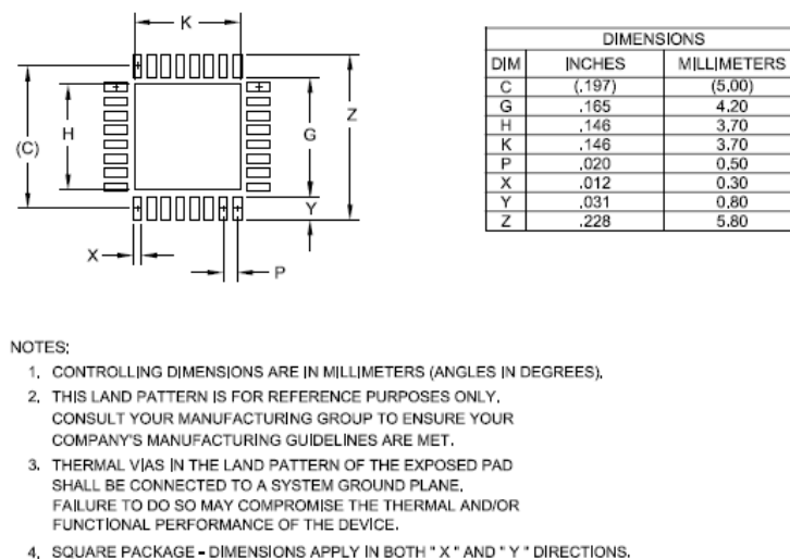
Figure 70 Land Pattern
