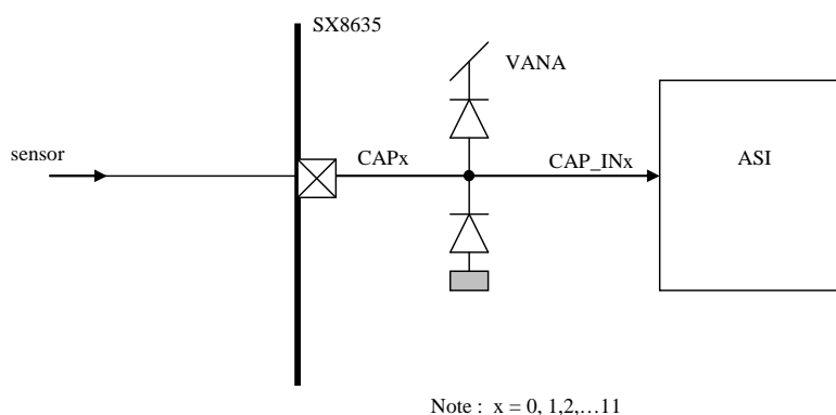
Figure 35 Simplified diagram of CAP0, CAP1, ..., CAP11
