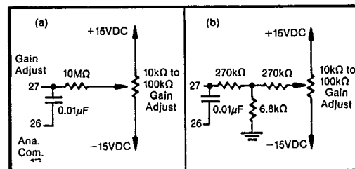
FIGURE 7. Two Methods of Connecting Optional Gain Adjust.
