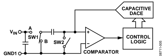
Figure 19. ADC Conversion Phase
