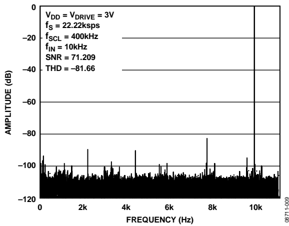
Figure 4. Typical FFT
