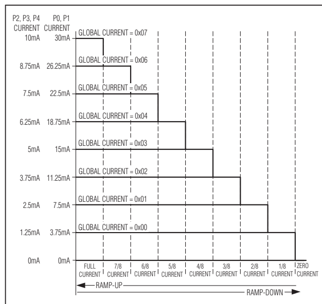
Figure 7. Global Current Modifies Ramp-Down Behavior
