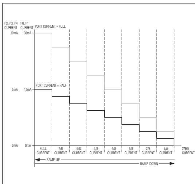
Figure 6. Output Fade DAC (Global Current = 0x07)
