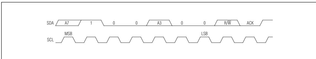
Figure 12. Slave Address
