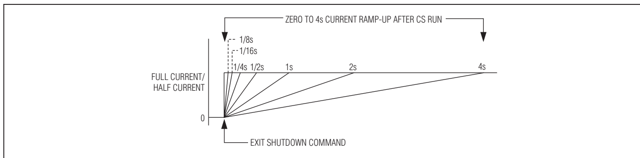
Figure 4. Ramp-Up Behavior
