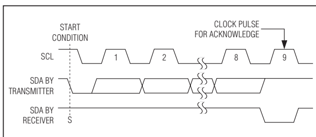
Figure 11. Acknowledge
