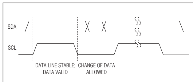
Figure 10. Bit Transfer
