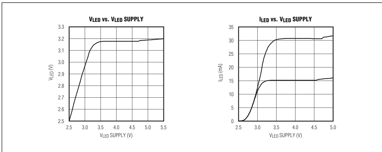
Figure 16. LED Brownout
