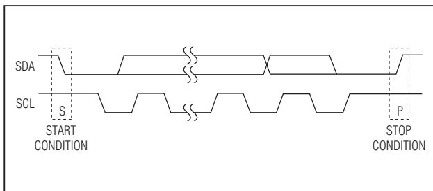
Figure 9. START and STOP Conditions
