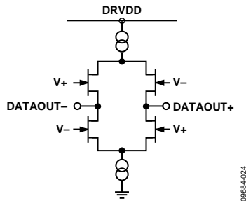
Figure 30. Equivalent LVDS Output Circuit
