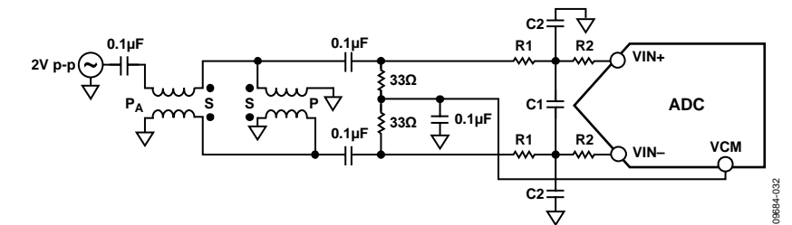
Figure 38. Differential Double Balun Input Configuration
