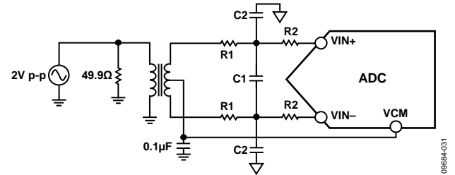
Figure 37. Differential Transformer-Coupled Configuration
