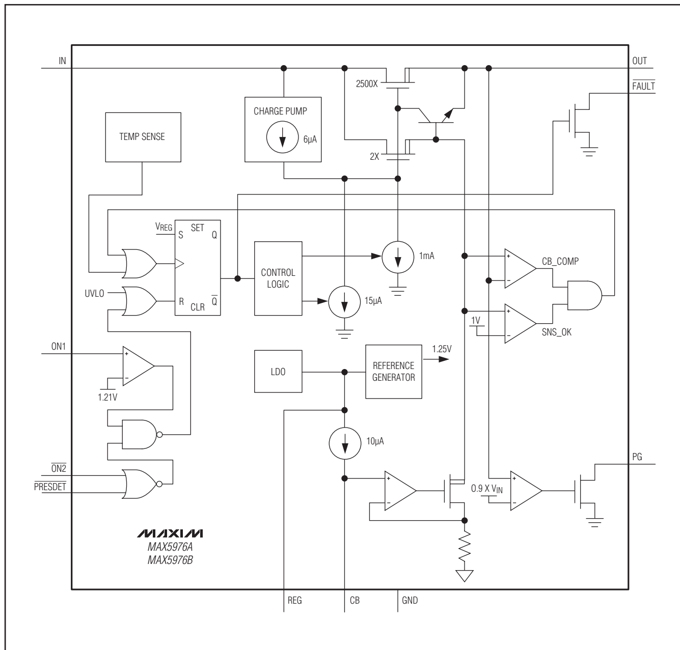
Functional Diagram
