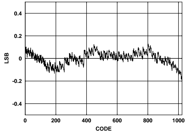
FIGURE 37. INTEGRAL NONLINEARITY
