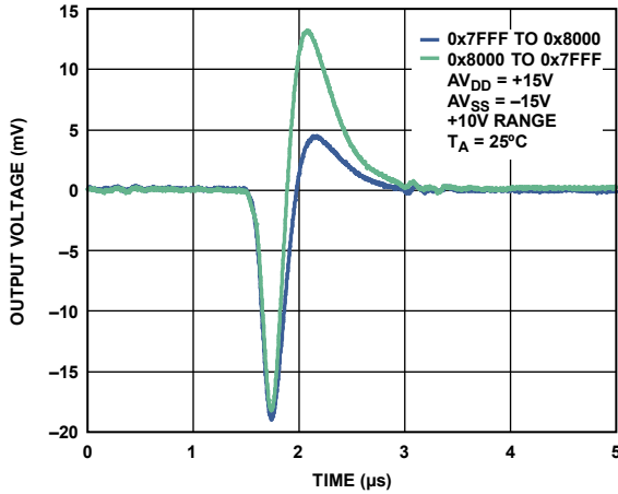
Figure 26. Digital-to-Analog Glitch
