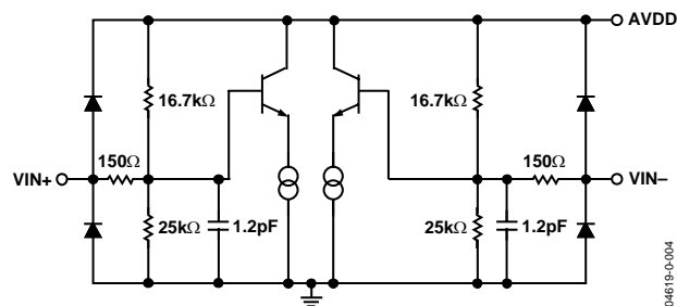
Figure 4. Analog Inputs
