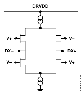
Figure 9. LVDS Data, DCO Outputs
