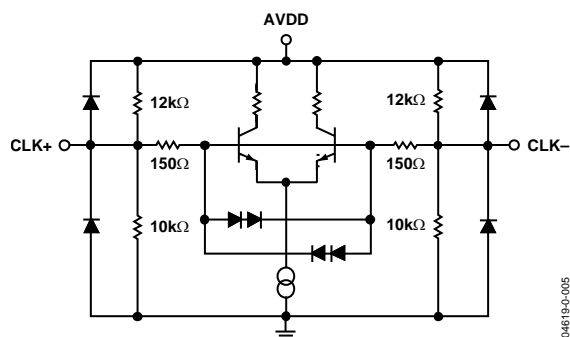
Figure 5. Clock Inputs
