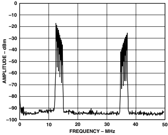
Figure 47. AD9775, Real DAC Output of Complex Input Signal Near Baseband (Negative Frequencies Only), Interpolation = 4x, Complex Modulation in AD9775 = -f_{DAC}/4
