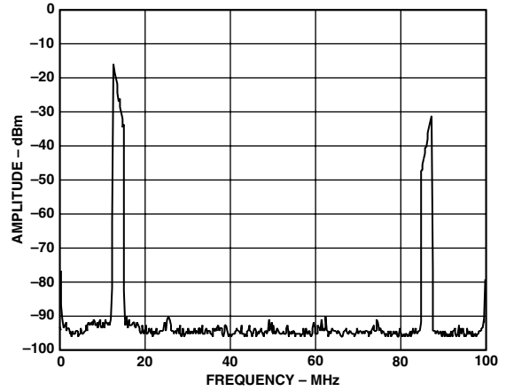
Figure 49. AD9775, Real DAC Output of Complex Input Signal Near Baseband (Positive Frequencies Only), Interpolation = 8x, Complex Modulation in AD9775 = +f_{DAC}/8
