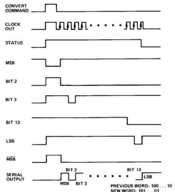
Figure 1. Timing Diagram
