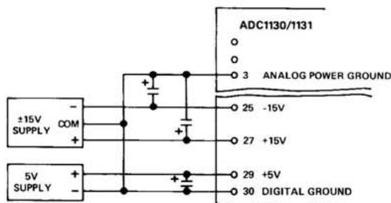
Figure 6. Power Supply and Grounding Connections
