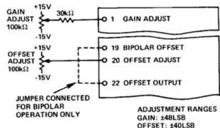
Figure 5. Adjustment Connections
