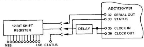
Figure 3. Serial Data Transmission
