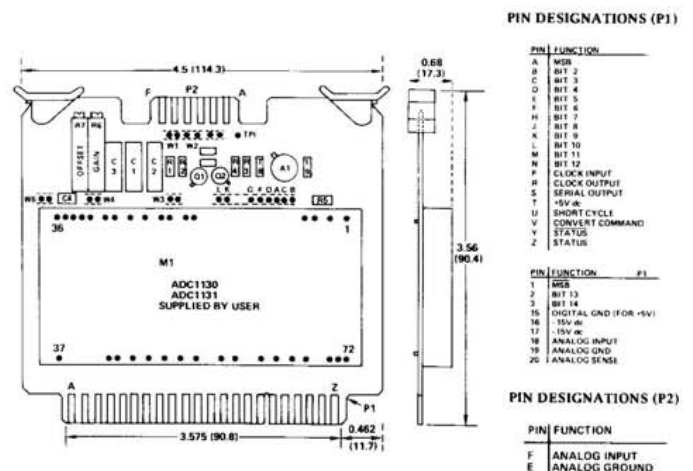
Figure 7. AC1578 Mounting Card
