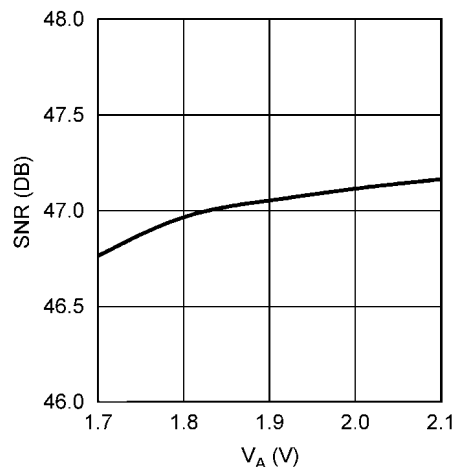
SNR vs. SUPPLY VOLTAGE
