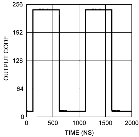
STEP RESPONSE
