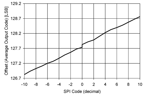
FIGURE 10. Extended Mode Offset Behavior
