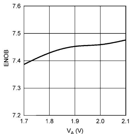
ENOB vs. SUPPLY VOLTAGE
