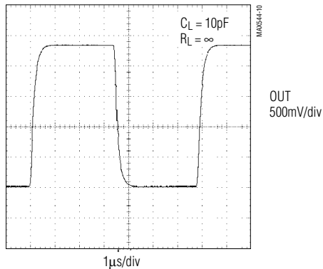
FULL-SCALE STEP RESPONSE (f SCLK = 10MHz)
