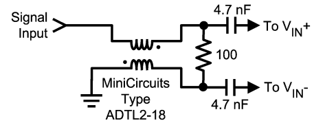
FIGURE 6. Single-Ended to Differential signal conversion with a balun-connected transformer
