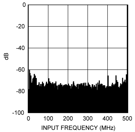
Spectral Response @ f_{IN} = 498\text{ MHz}
