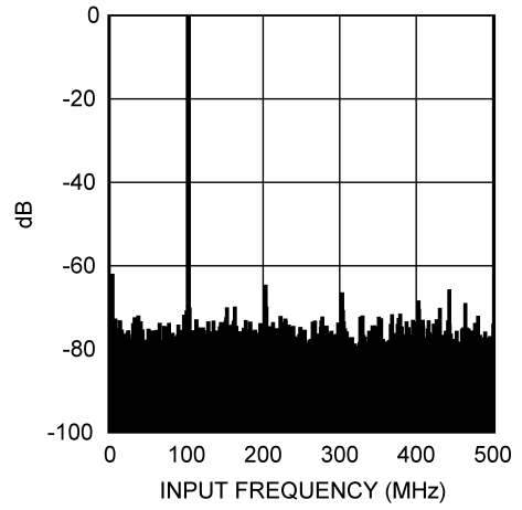
Spectral Response @ f_{IN} = 100\text{ MHz}
