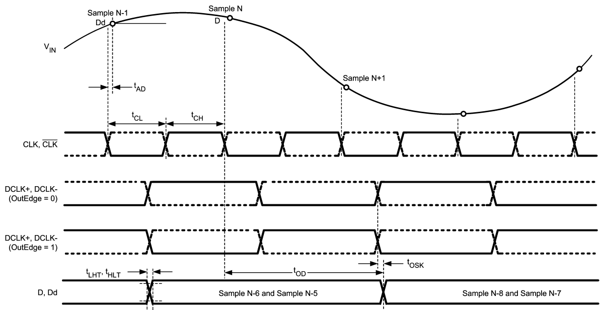
FIGURE 3. ADC081000 Timing
