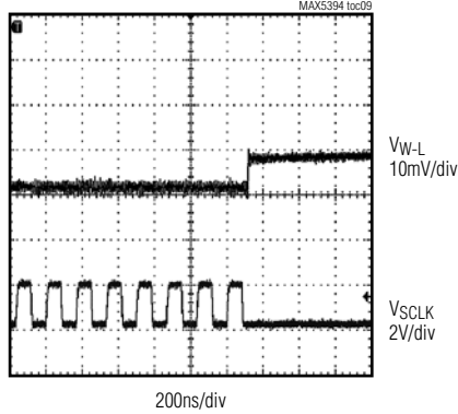
TAP-TO-TAP SWITCHING TRANSIENT (CODE 127 TO 128 10kΩ)
