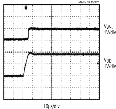
POWER-ON TRANSIENT (50kΩ)
