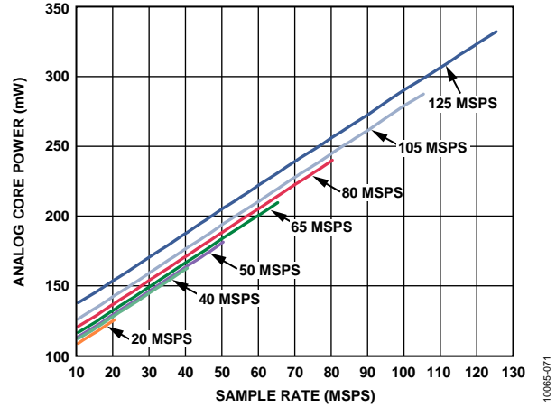
Figure 69. Analog Core Power vs. f_{SAMPLE} for f_{IN} = 10.3 MHz
