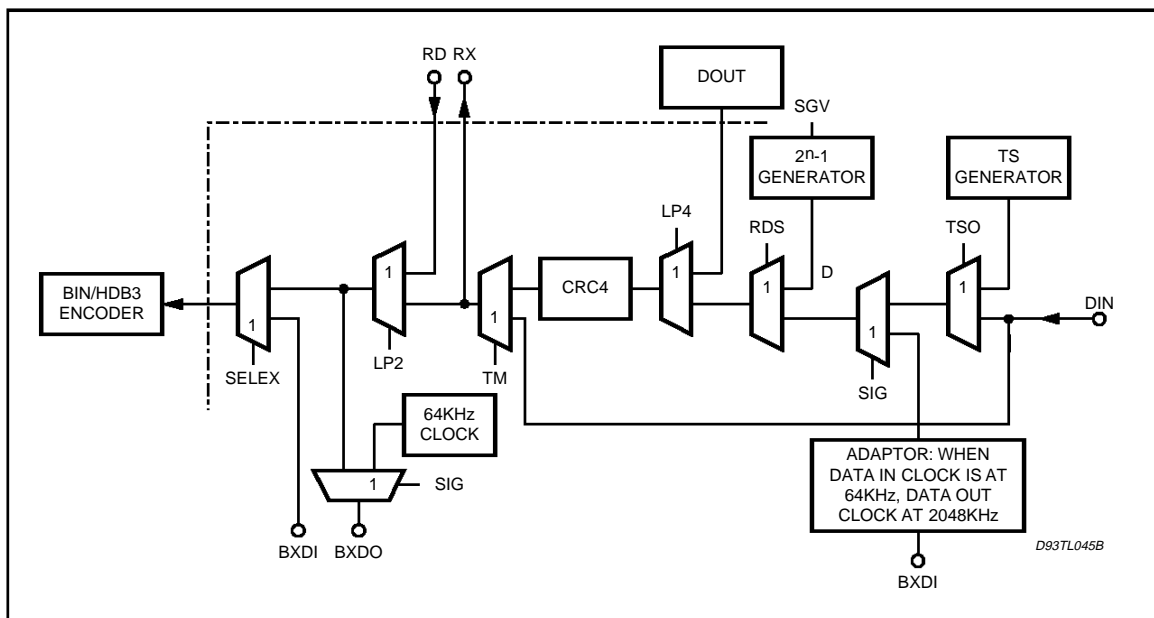
Figure 2: Transmitter Diagram
