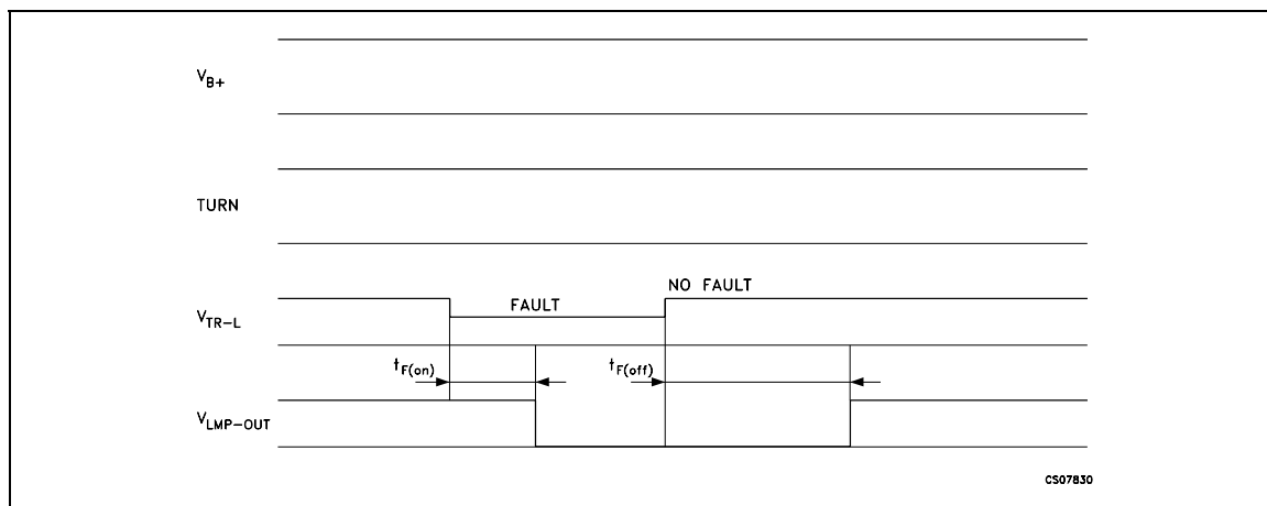
Figure 3 : Fault indication on and off timing diagram
