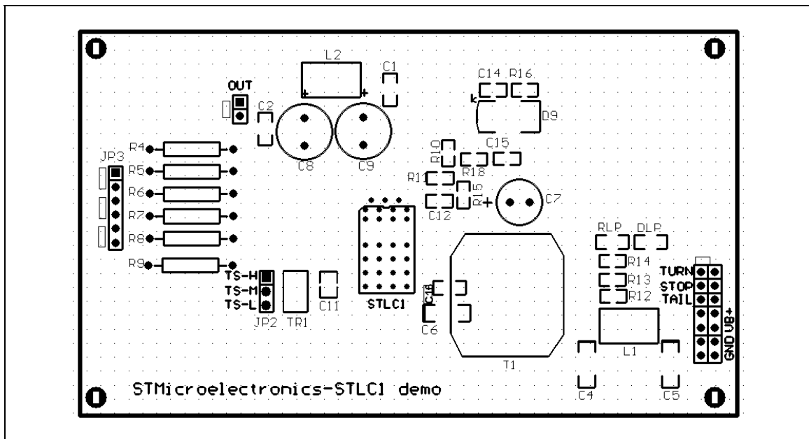
Figure 16 : PCB Components outline
