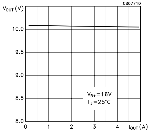
Figure 5 : Output Voltage vs Output Current
