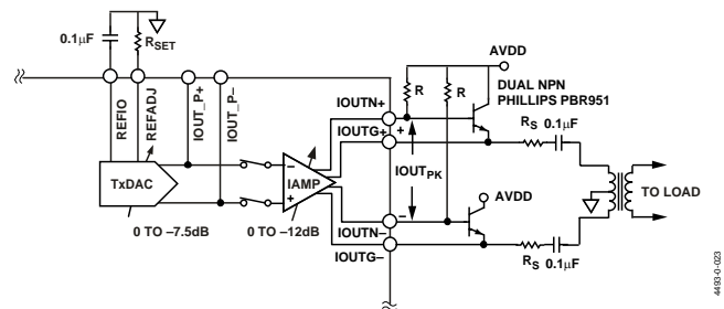
Figure 65. Voltage-Mode Operation
