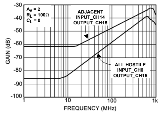
FIGURE 12. CROSSTALK - A_V = 2
