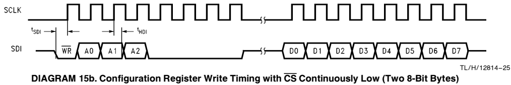
DIAGRAM 15b. Configuration Register Write Timing with \overline{CS} Continuously Low (Two 8-Bit Bytes)
