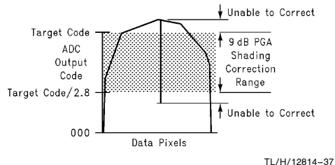
FIGURE 10. CCD Input Signal Range Too Wide
