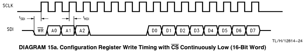
DIAGRAM 15a. Configuration Register Write Timing with \overline{CS} Continuously Low (16-Bit Word)
