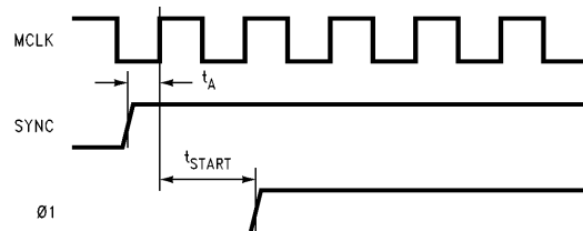
DIAGRAM 3. Timing for Start of Line Scan
