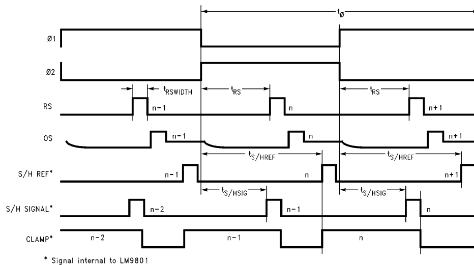
DIAGRAM 8. CCD Timing (Even/Odd CCDs)
