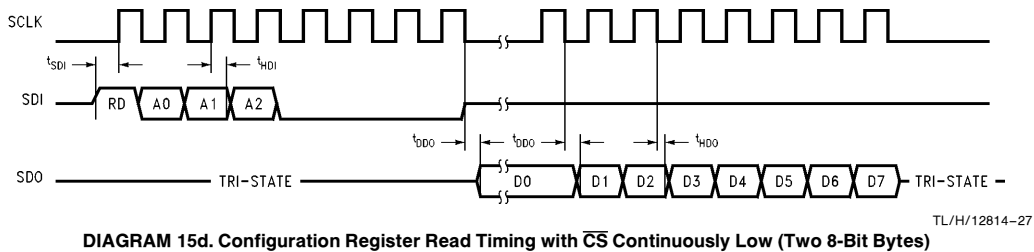
DIAGRAM 15d. Configuration Register Read Timing with \overline{CS} Continuously Low (Two 8-Bit Bytes)
