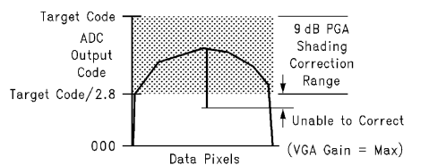
FIGURE 11. CCD Input Signal Too Weak
