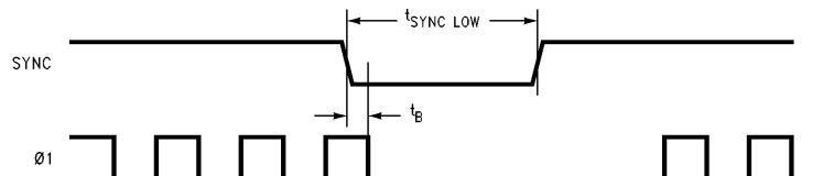
DIAGRAM 4. Timing for End of Line/Start of Next Line
