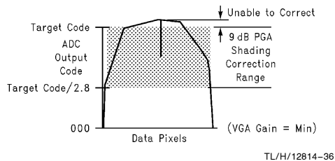
FIGURE 9. CCD Input Signal Too Strong
