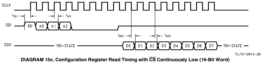
DIAGRAM 15c. Configuration Register Read Timing with \overline{CS} Continuously Low (16-Bit Word)
