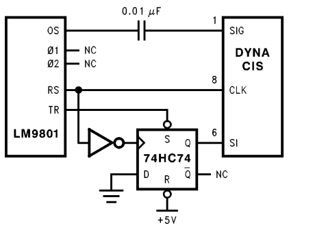
FIGURE 19. Minimum CIS Interface
