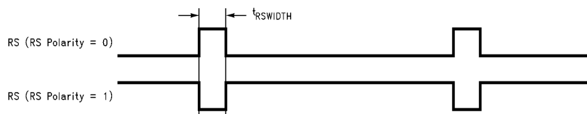
DIAGRAM 6. RS Pulse Polarity
