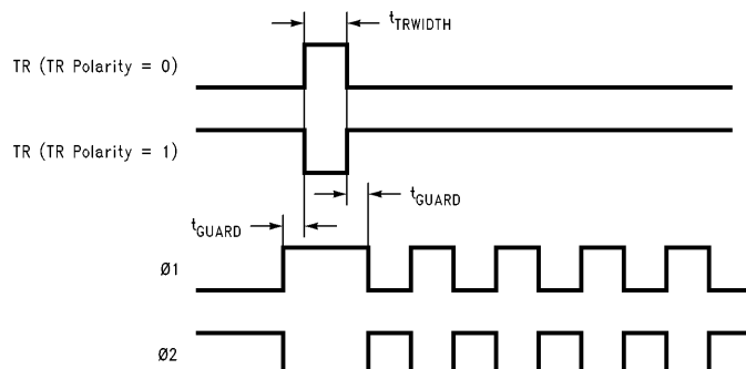
DIAGRAM 5. TR Pulse Timing
