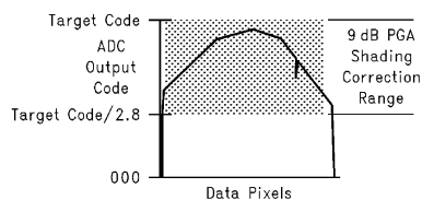
FIGURE 7. CCD Input Signal In Range
