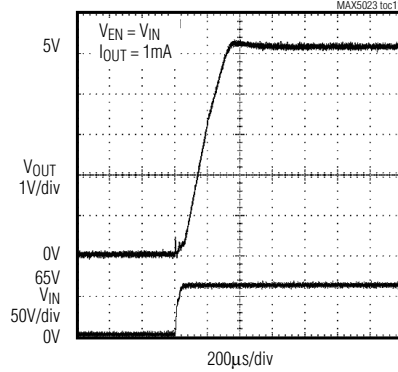
STARTUP RESPONSE
