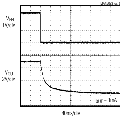
SHUTDOWN RESPONSE
