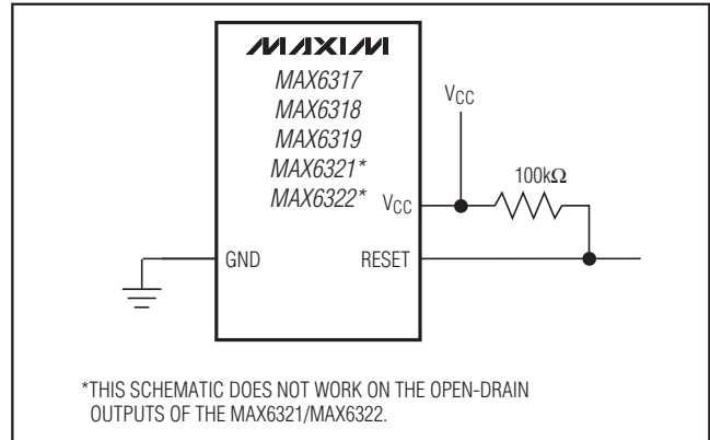
Figure 9. Ensuring \overline{\text{RESET}} Valid to V_{CC} = 0V on Active-High Push/Pull Outputs
