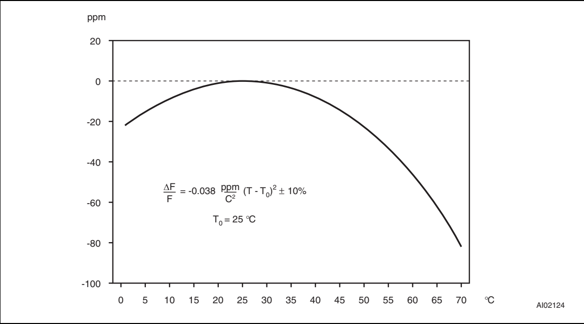
Figure 8. Crystal accuracy across temperature
