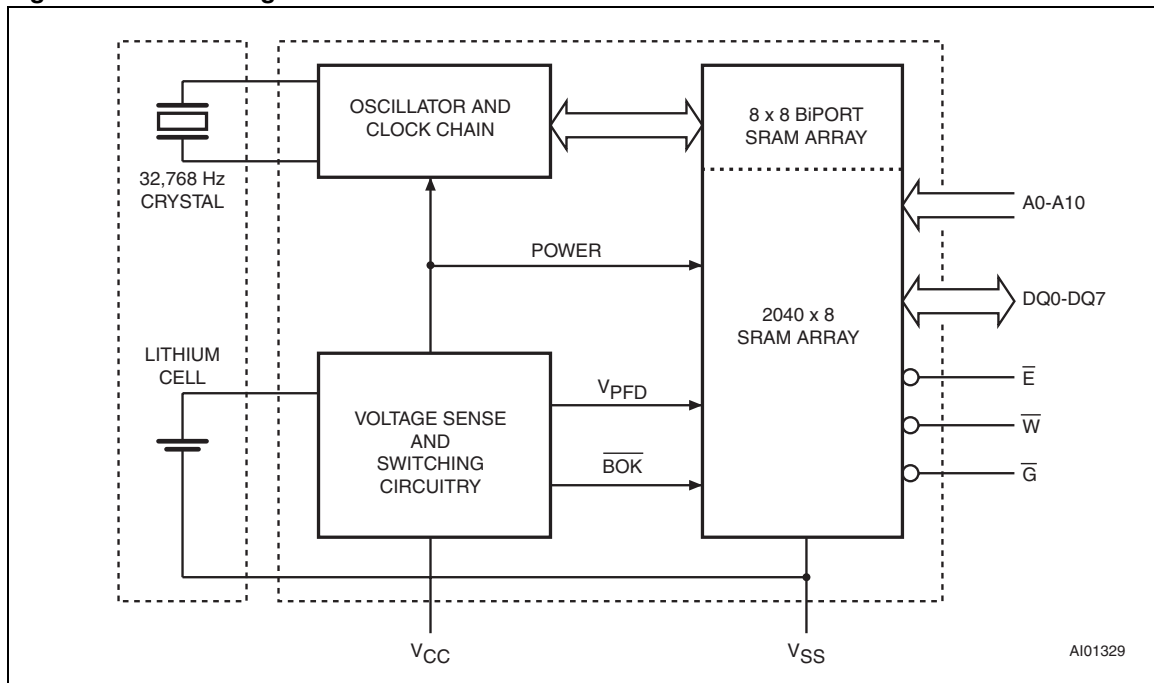
Figure 3. Block diagram
