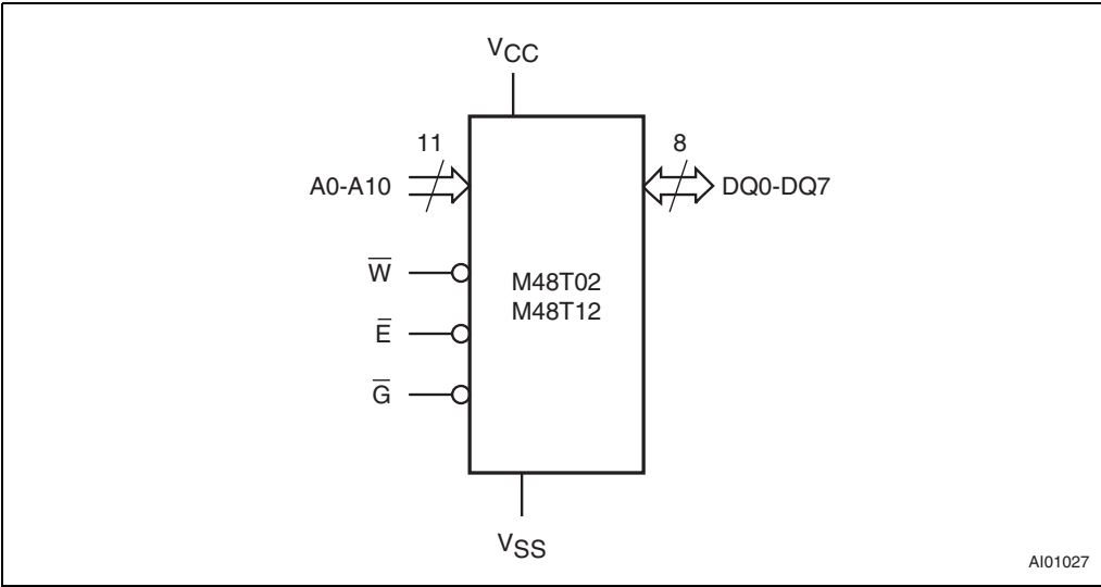
Figure 1. Logic diagram
