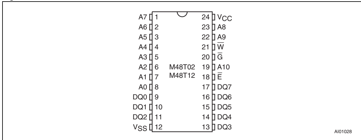
Figure 2. DIP connections
