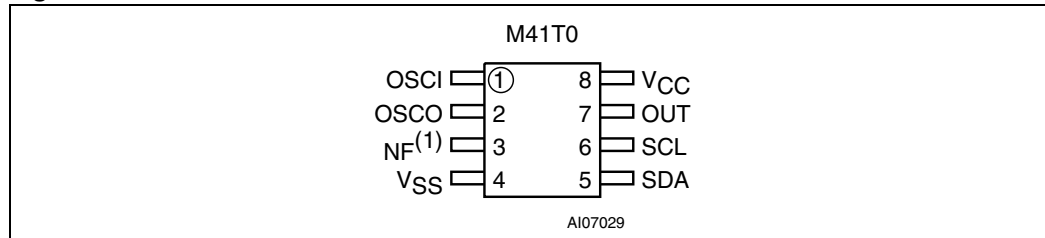
Figure 2. SOIC connections
