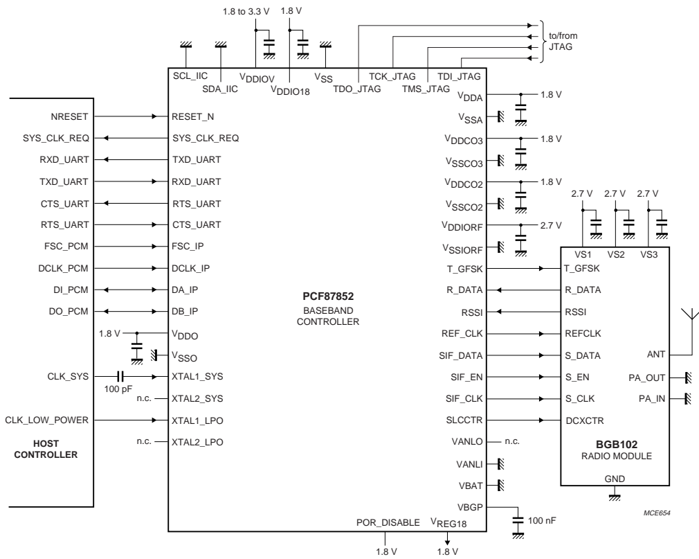
Fig 2. Application example of hosted Bluetooth system with PCF87852 and BGB102 (or BGB101) RF module.
