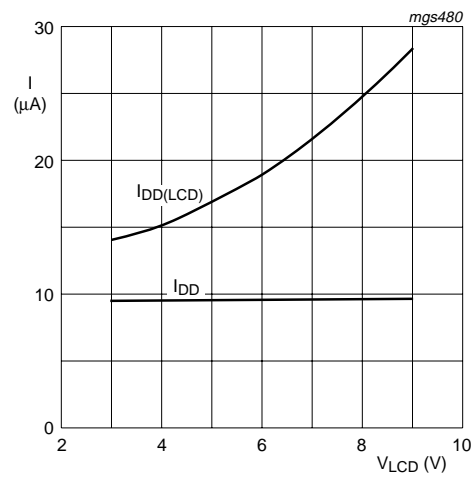
Fig 25. Supply current as a function of LCD supply voltage
