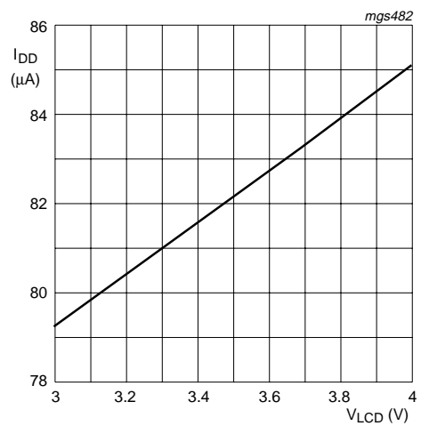
Fig 27. Supply current as a function of LCD supply voltage
