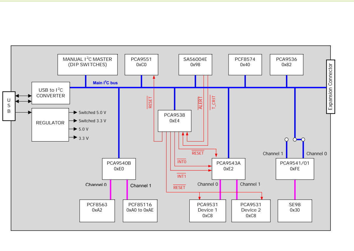
Fig 3. I2C Demonstration Board 2005-1 block diagram
