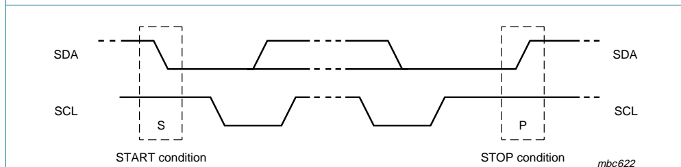
Fig 30. Definition of START and STOP conditions
