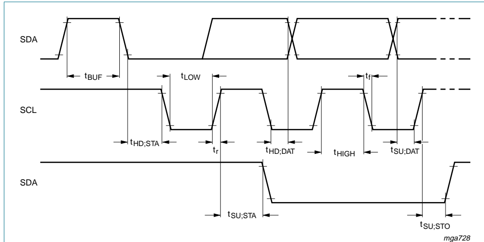
Fig 34. I 2 C-bus timing diagram
