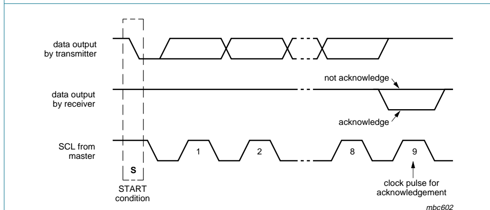
Fig 31. Acknowledgement on the I 2 C-bus
