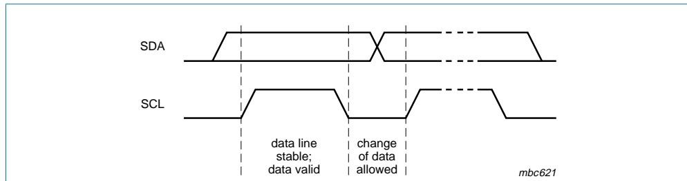
Fig 29. Bit transfer
