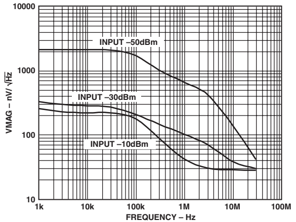
TPC 23. Magnitude Output Noise Spectral Density, P_{INPA} = P_{INPB} = -10 \text{ dBm} , -30 \text{ dBm} , -50 \text{ dBm} , with Filter Capacitor, C = 1 \text{ nF}
