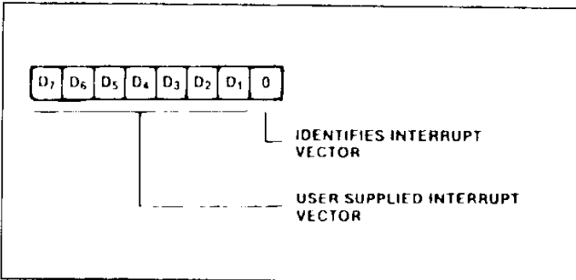
Figure 7 : I/O Register Control Word.
