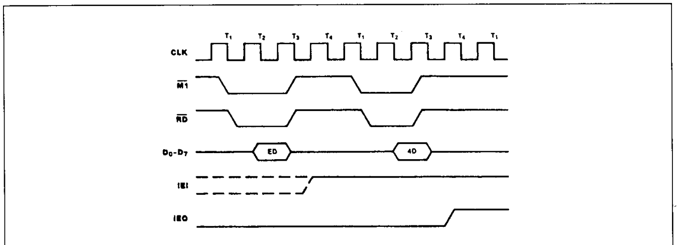
Figure 18 : Return From Interrupt.
