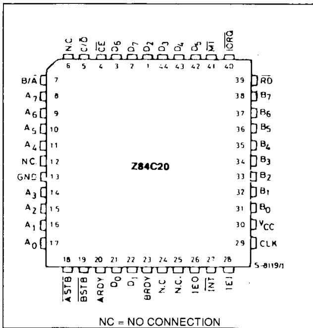
Figure 2 : Chip Carrier Pin Configuration.
