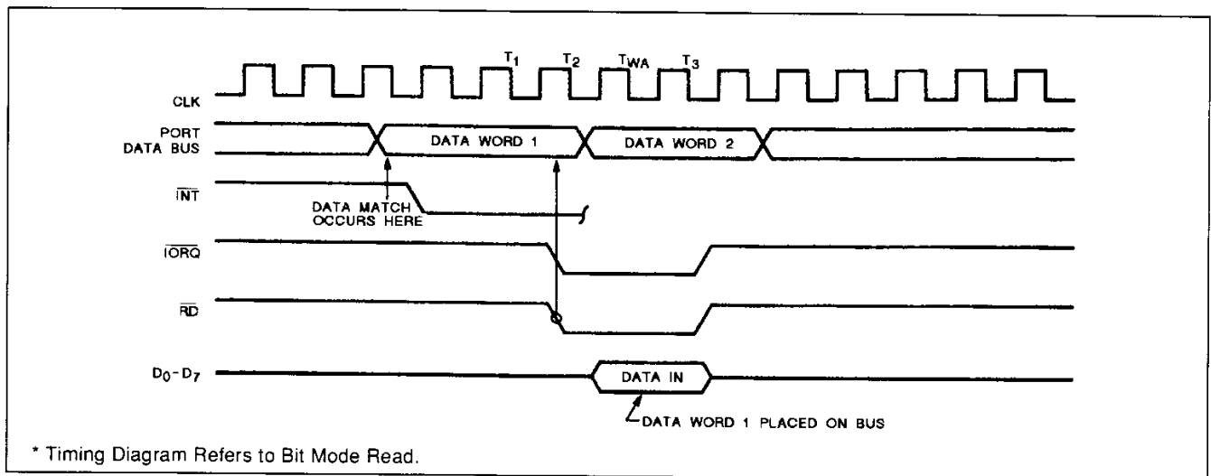
Figure 16 : Mode 3 Bit Mode Timing.
