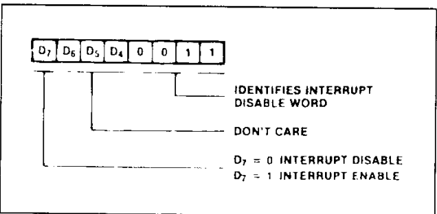
Figure 10 : Interrupt Disable Word.
