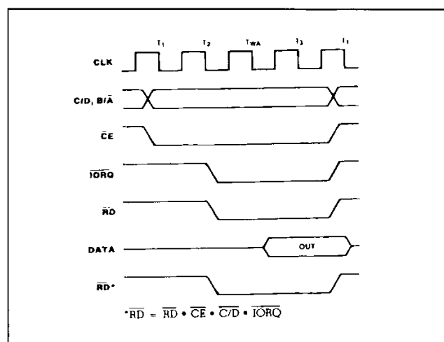
Figure 12 : Read Cycle Timing.
