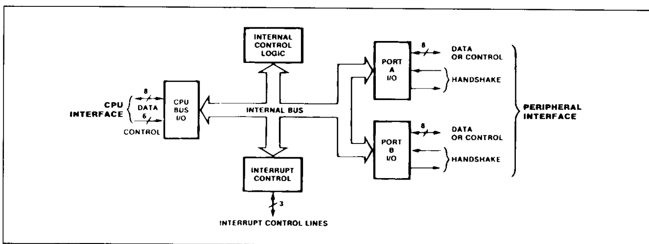
Figure 3 : Block Diagram.
