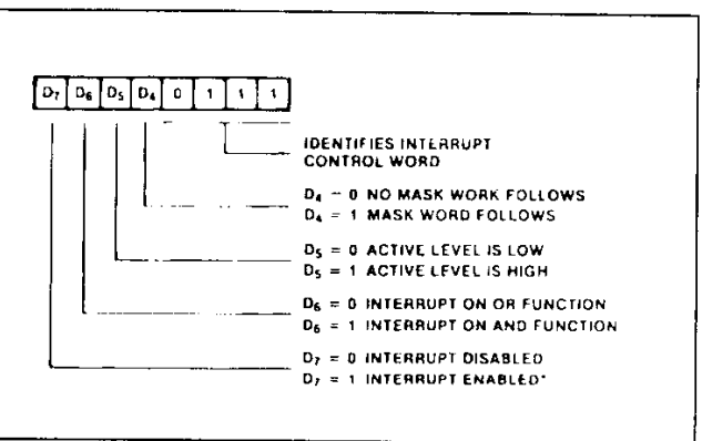
Figure 8 : Interrupt Control Word.
