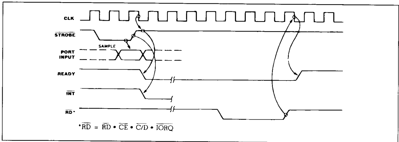
Figure 15 : Mode 2 Bidirectional Timing.
