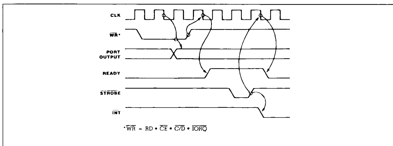
Figure 13 : Mode 0 Output Timing.
