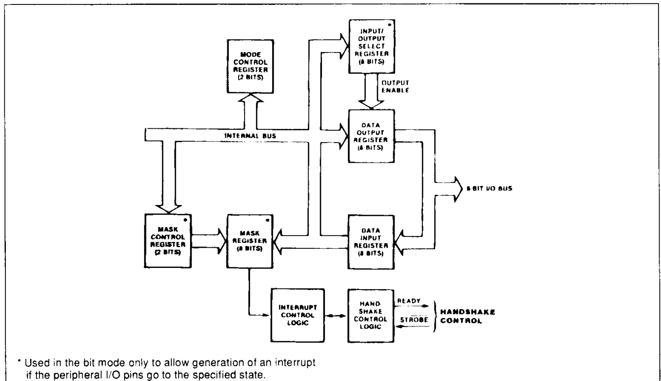
Figure 4 : Typical Port I/O Block Diagram.
