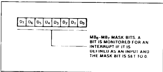
Figure 10 : Interrupt Disable Word.
