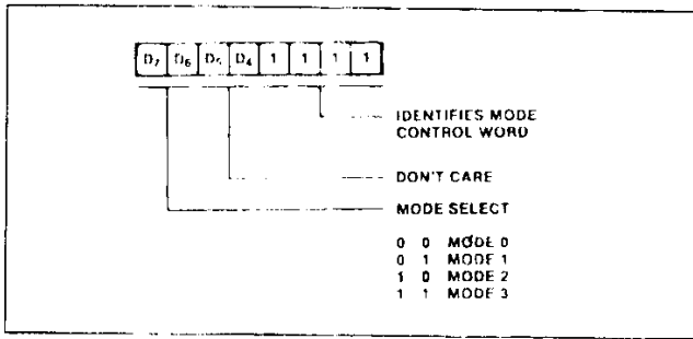
Figure 6 : Interrupt Vector Word.
