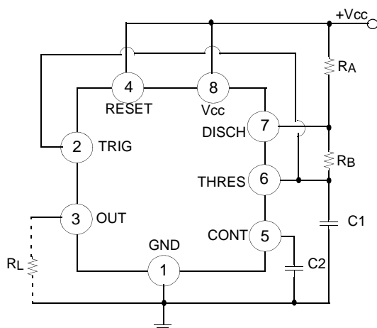
Figure 5. Astable Circuit
