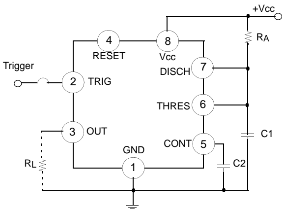
Figure 1. Monostable Circuit
