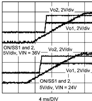
Softstart Waveforms (No-Load Both Channels)
