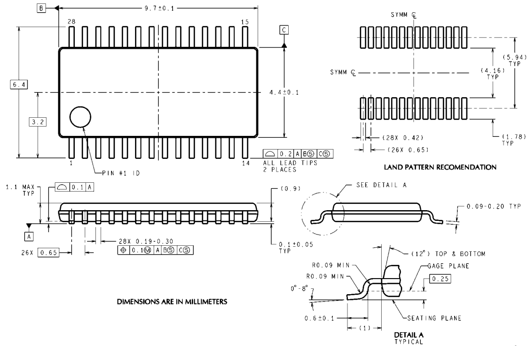
28-Lead TSSOP Package Order Number LM5642MTC, LM5642XMT NS Package Number MTC28
