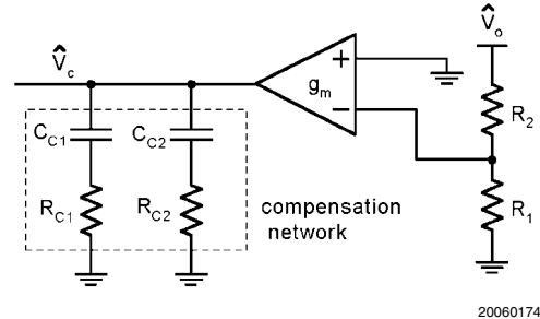
FIGURE 13. Compensation Network
