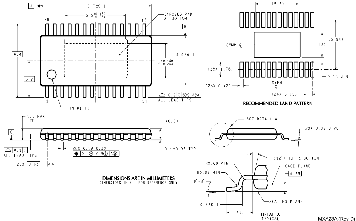
28-Lead eTSSOP Package Order Number LM5642MH, LM5642XMH NS Package Number MXA28A
