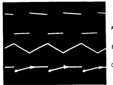
A = Switch Voltage (LX) 5V/div (4.8V to -5.3V) B = Inductor Current, 500mA/div C = Output Voltage Ripple, 50mV/div TIME = 2µs/div CIRCUIT OF FIG. 1 V IN = +5V T A = +25°C
