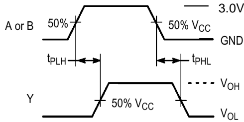
Figure 4. Switching Waveforms
