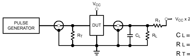
Figure 6. Test Circuit
