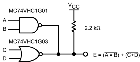
Figure 7. Complex Boolean Functions
