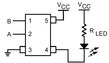
Figure 8. LED Driver
