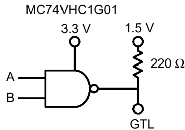
Figure 9. GTL Driver
