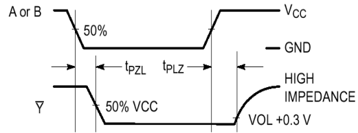
Figure 5. Switching Waveforms
