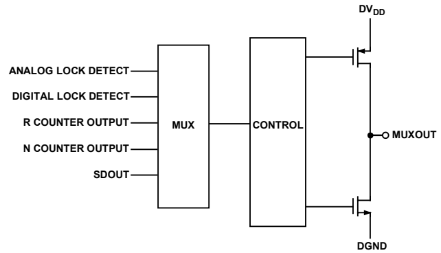
Figure 15. MUXOUT Circuit
