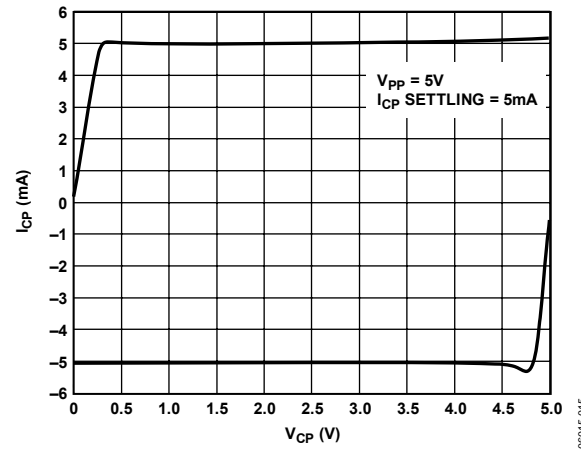
Figure 9. Charge Pump Output Characteristics
