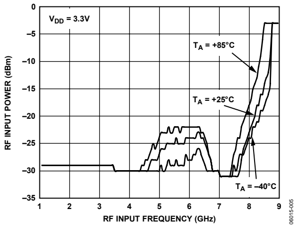
Figure 6. RF Input Sensitivity
