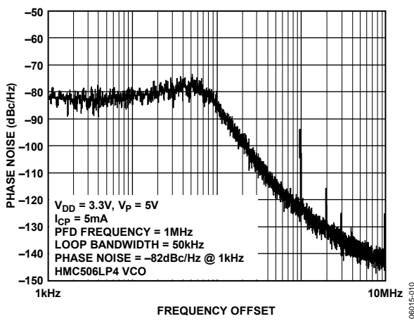
Figure 7. Phase Noise at 7.9 GHz Phase Noise
