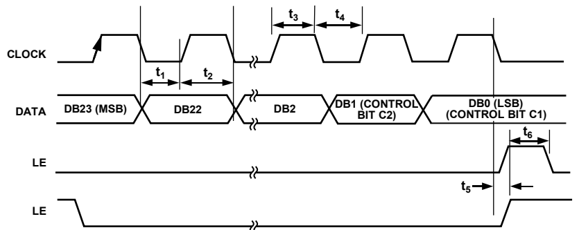
Figure 2. Timing Diagram
