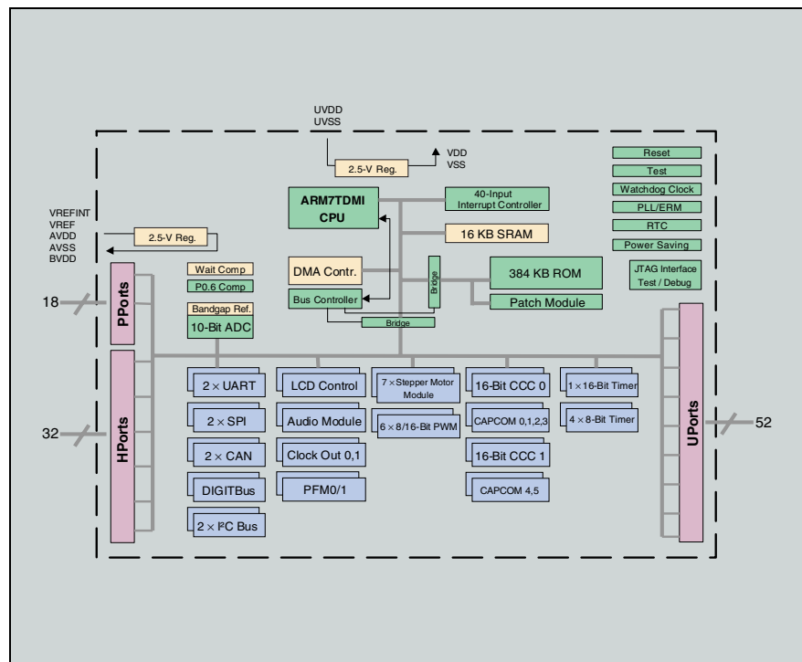
Fig. 2: Block diagram of the CDC 3272G
