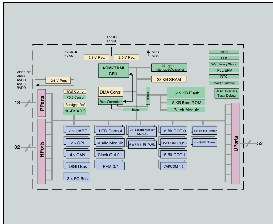
Fig. 2: Block diagram of the CDC 3207G
