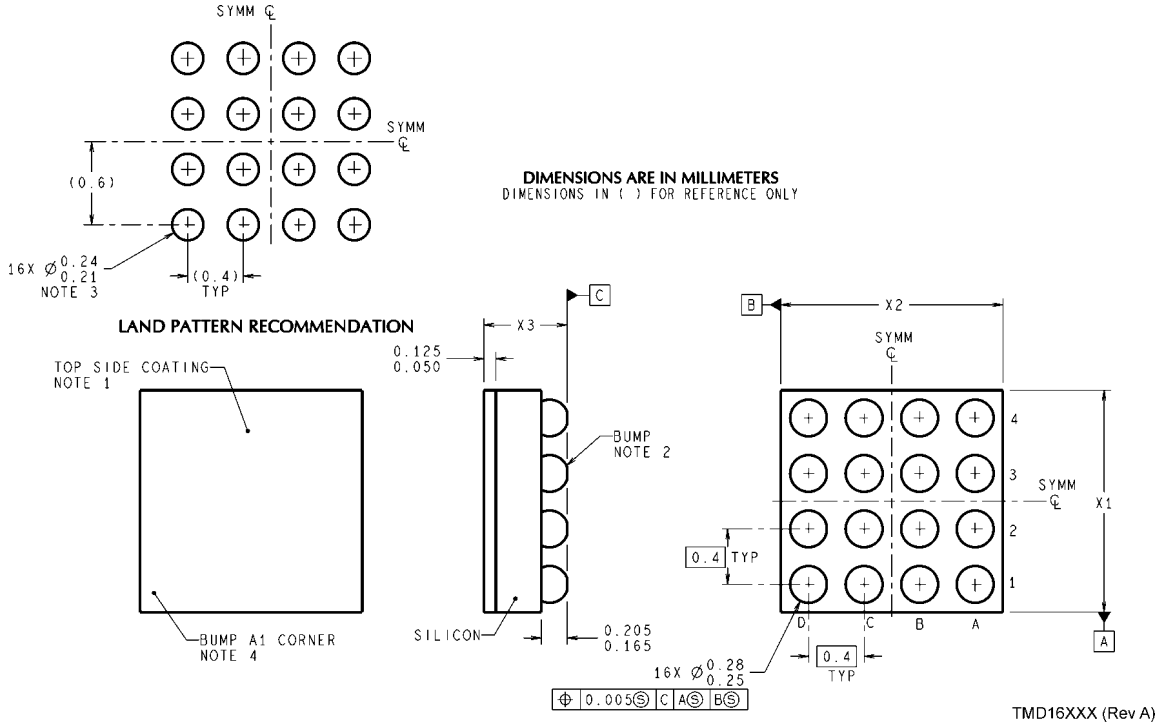
16-Bump micro SMD NS Package Number TMD16AAA X1 = 1.615 ± 0.030 mm, X2 = 1.615 ± 0.030 mm, X3 = 0.600 ± 0.075 mm
